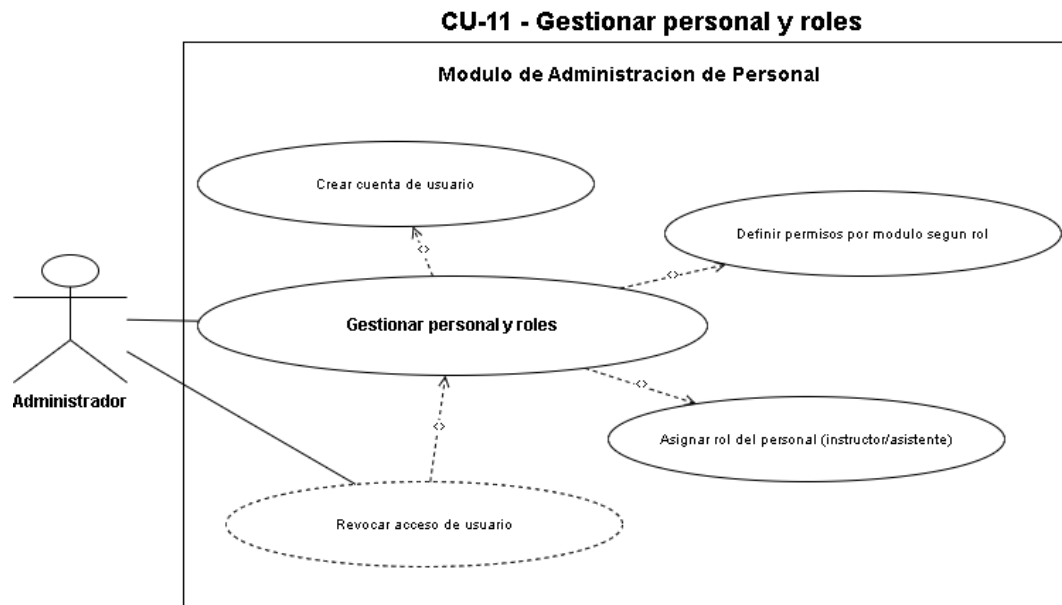
Figura 17: CU- 11Gestionar Personal y Roles
